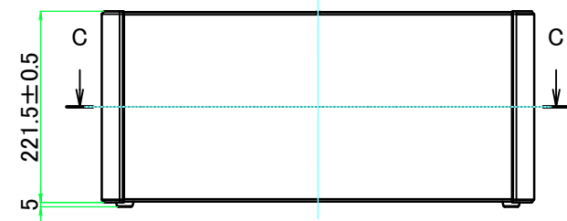
A view
